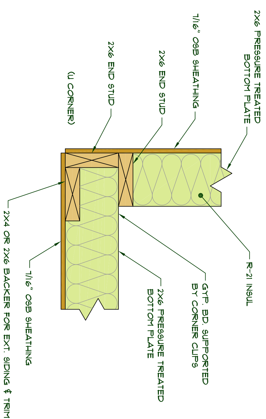
6 3 STUD U-CORNER DETAIL SCALE 3/4"=1'-0"
